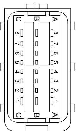
Sicma 24-pole pin header HCCPHPE24BKA90F black
