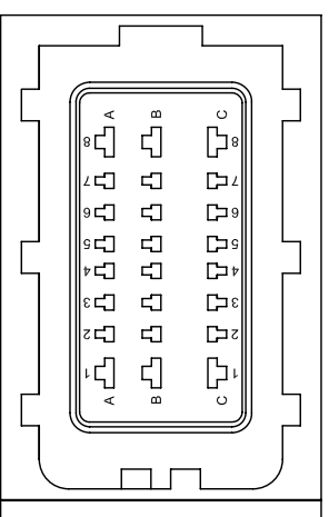
Sicma 24-pole female housing 211PC249S0005 black
