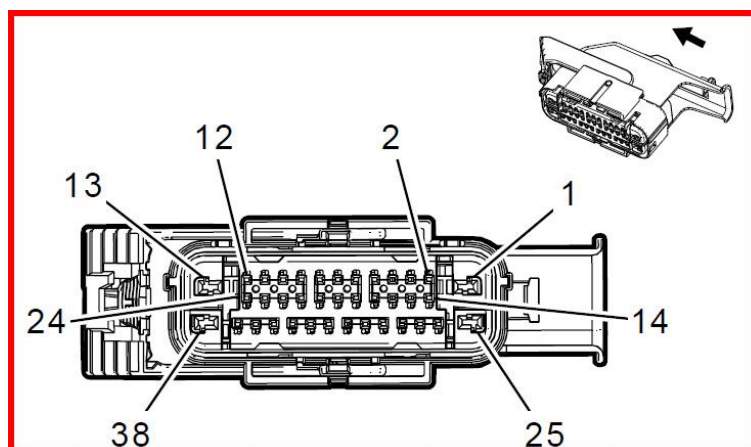
Location Chassis Control Module GMC Savana
