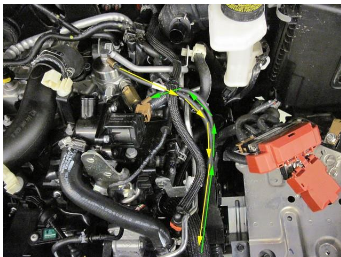
Mount hoses from high pressure pump to FSU & FRU. Mount protection.
