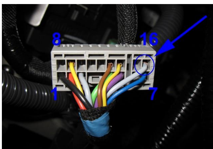
Wake up: Connector BP GREY , pos 16
