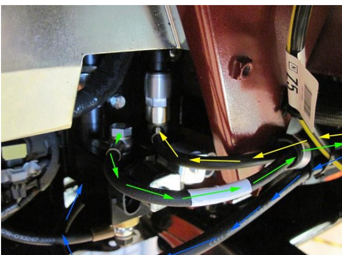
Mount hoses from high pressure pump to FSU & FRU.
