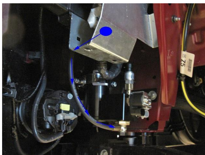
Connect hose from boost pump to FSU.
