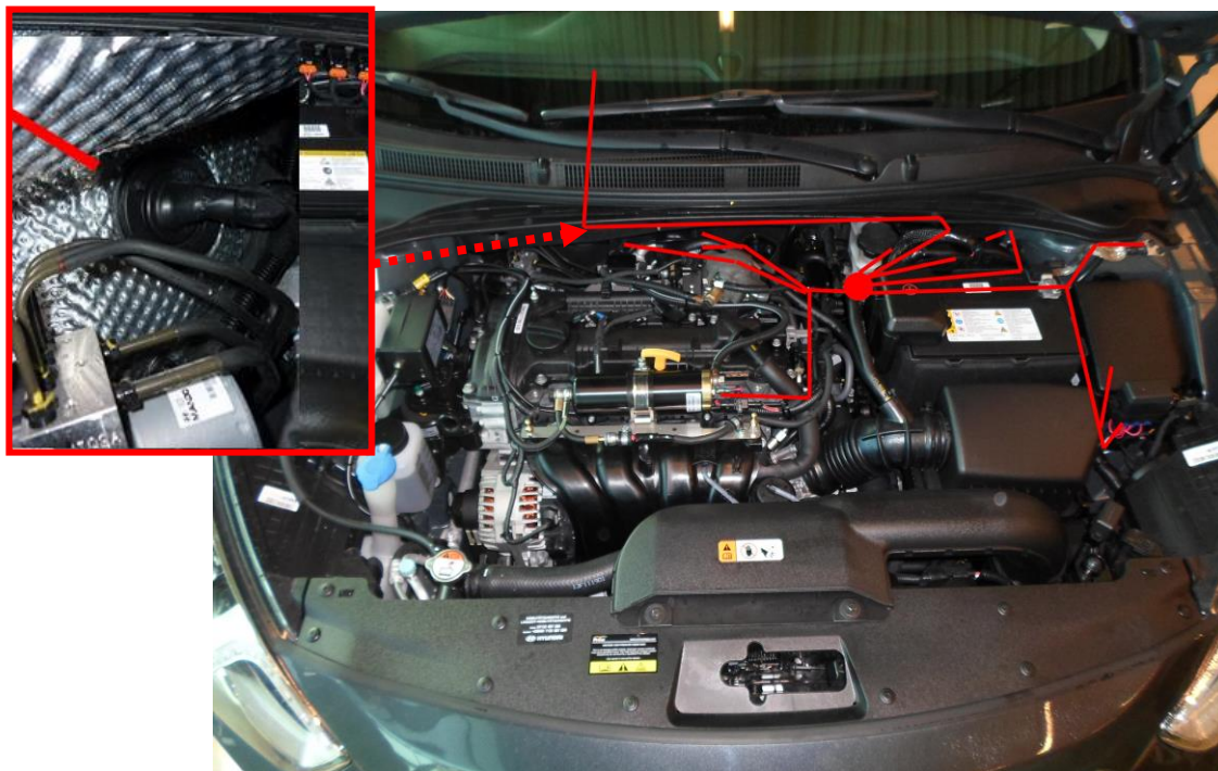
Wiring harness the DLM system.
