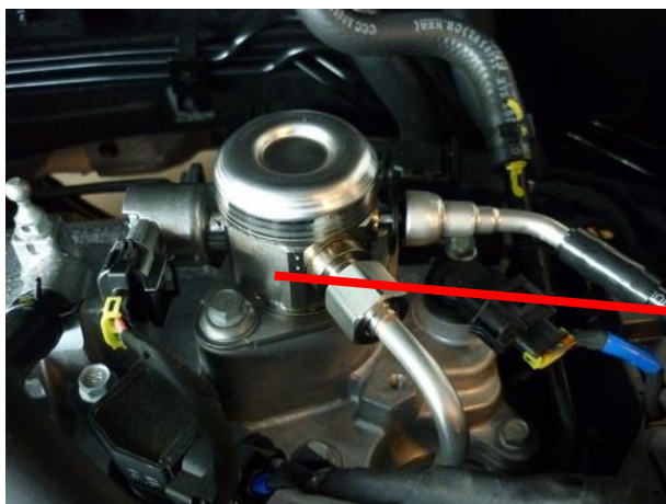
Remove the original high pressure pump.
