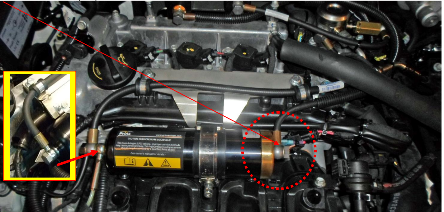
3 rd Generation Boostpump
