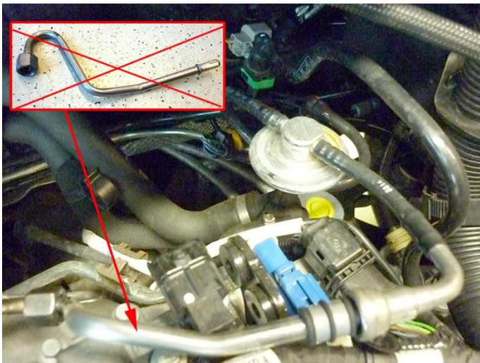
Remove low pressure petrol line ( not used )
