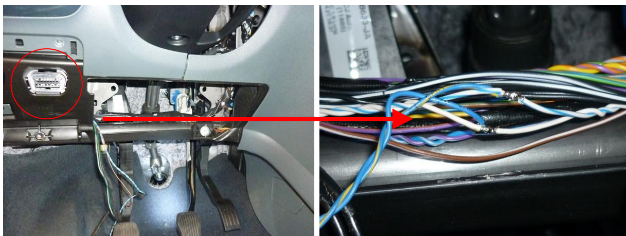
EOBD ( CAN )
