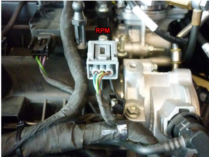
Tect connector: under HPPump housing:
