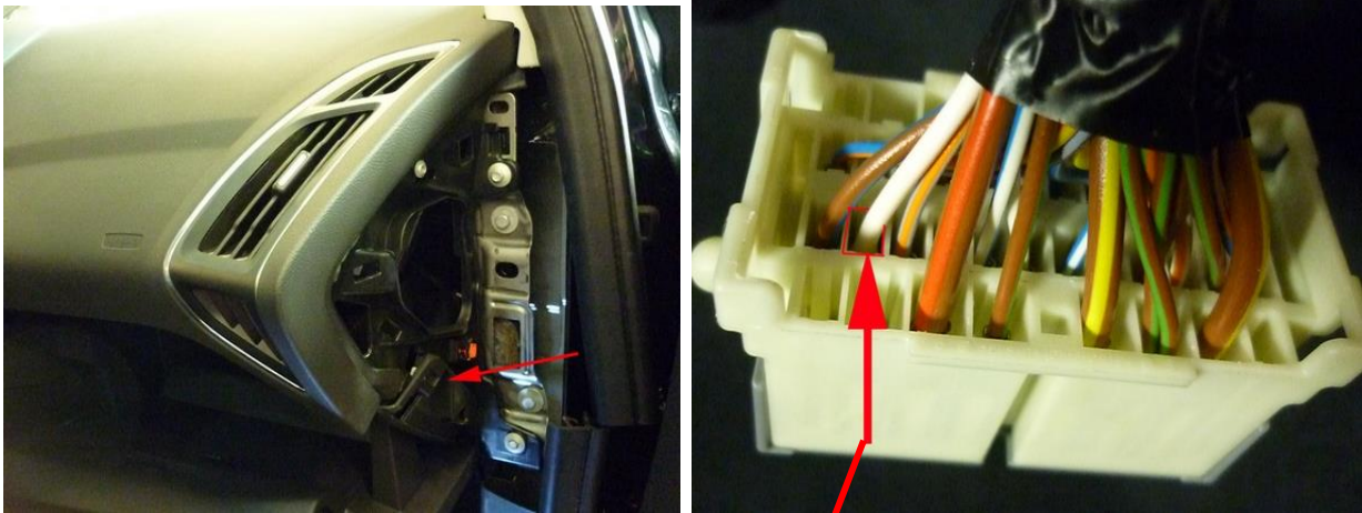
White wire = PWM 56
