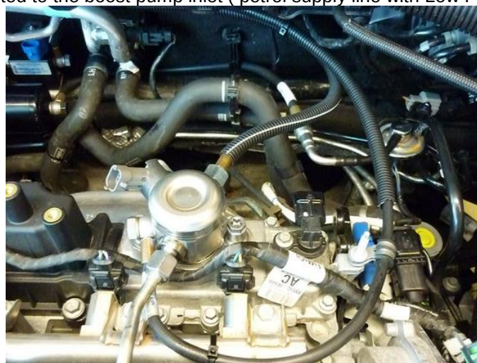
Original hose connected to the boost pump inlet ( petrol supply line with Low Pressure petrol sensor )
