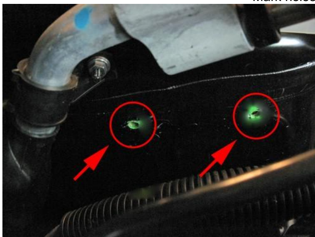
Drill holes Ø6,5mm for mounting boost pump bracket.
